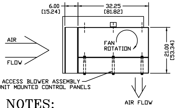
END VIEW (CONTROL PANEL REMOVED)
