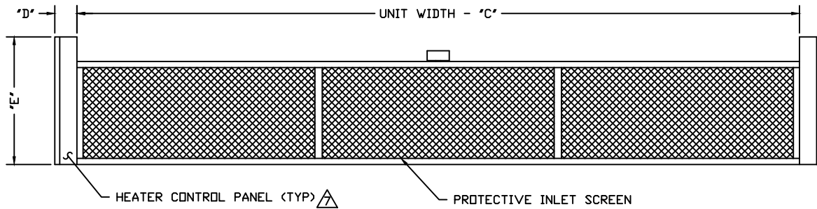
BOTTOM VIEW
