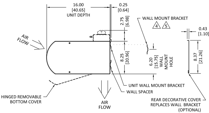
END VIEW
