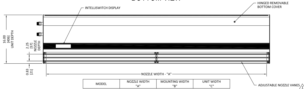
BOTTOM VIEW
