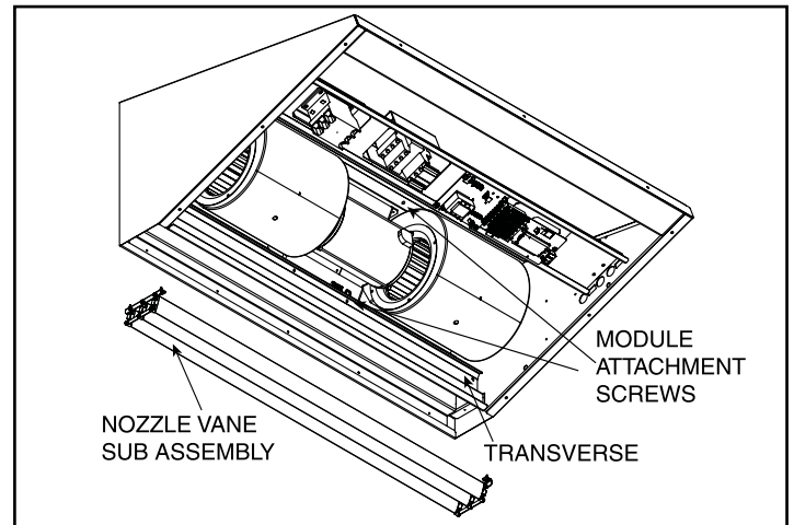
ARCHITECTURAL ELITE 10 - REPLACING FANS / MOTORS
