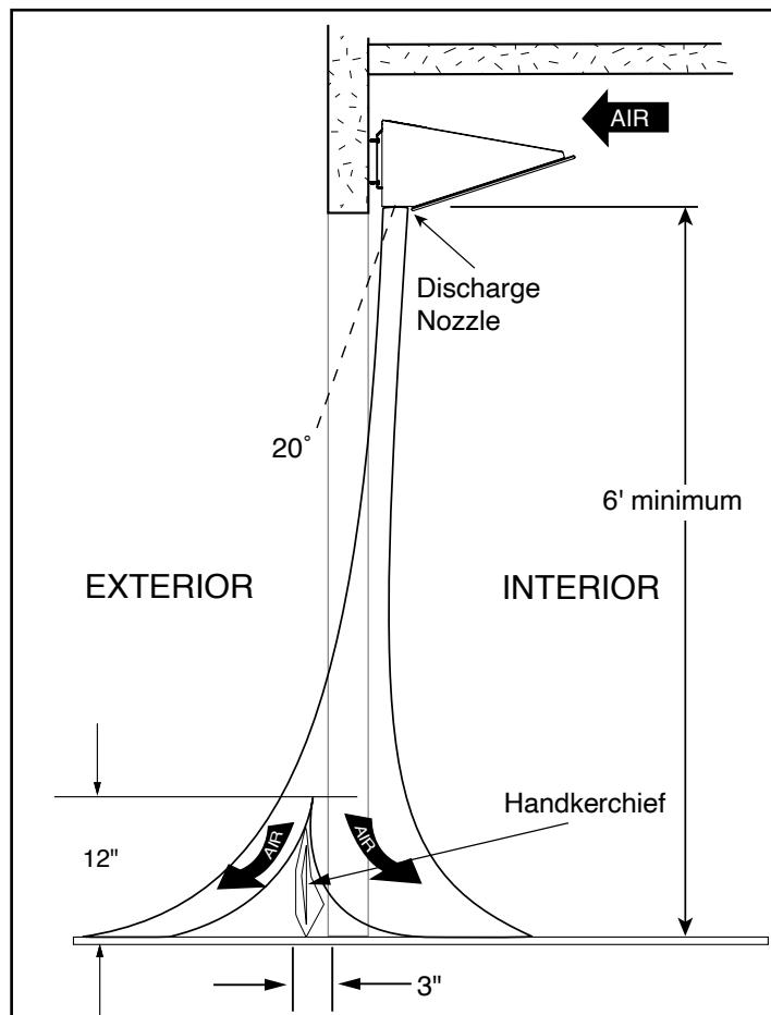
Figure 9 - Air Stream Adjustment
