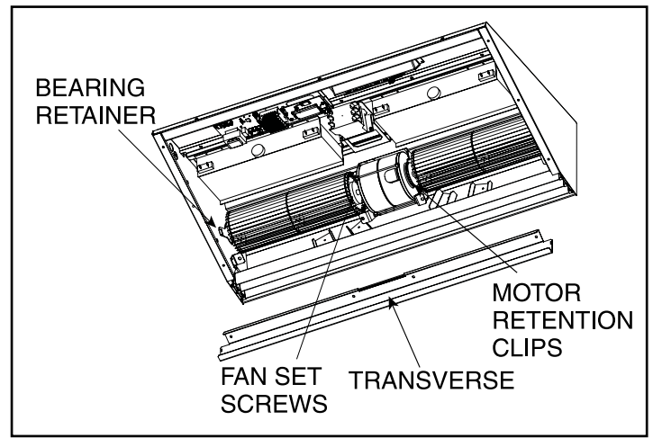
ARCHITECTURAL ELITE 8 - REPLACING FANS / MOTORS
