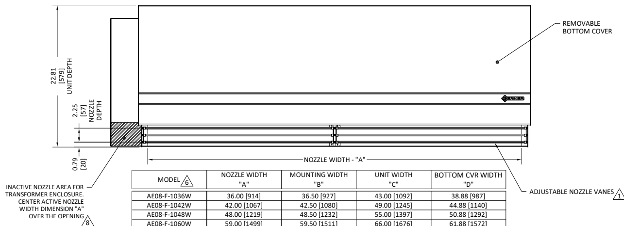
BOTTOM VIEW
